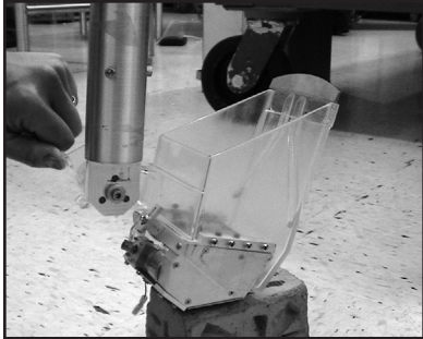
Close up of the scoop and other instruments at the end of the RA. Photo courtesy of NASA, UA Phoenix website
